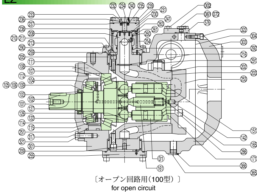
〔クローズド回路用(200型)〕 for closed circuit
