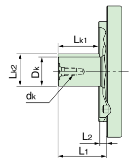
●SAEキー入力軸形状 Keyed shaft
