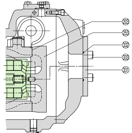
〔吸入弁付回路用(400型)〕 for semi-closed circuit
